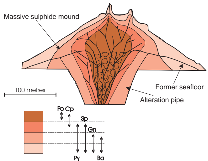
FIGURE 20. Mineral zonation commonly observed within VMS deposits; this zoning is largely a function of hydrothermal fluid temperature and composition. Temperature gradient results in the zoning of sulphide minerals within both the discordant stockwork zone and the conformable sulphide mound. From Lydon (1984).
