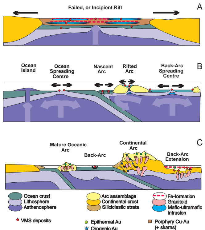
FIGURE 11. There are three principal tectonic environments in which VMS deposits form, each representing a stage in the formation of the Earth's crust. (A) Early Earth evolution was dominated by mantle plume activity, during which numerous incipient rift events formed basins characterized by early ocean crust in the form of primitive basalts and/or komatiites, followed by siliciclastic infill and associated Fe-formation and mafic-ultramafic sills. In the Phanerozoic, similar types of incipient rifts formed during transpressional, back-arc rifting (Windy Craggy). (B) The formation of ocean basins was associated with the development of ocean spreading centers along which mafic-dominated VMS deposits formed. The development of subduction zones resulted in oceanic arc formation with associated extensional domains in which bimodal mafic, bimodal felsic, and mafic-dominated VMS deposits formed. (C) The formation of mature arc and ocean-continent subduction fronts resulted in successor arc and continental volcanic arc assemblages that host most of the felsic-dominated and bimodal siliciclastic deposits. Thin black arrows represent direction of extension and thick, pale arrows represent mantle movement. Modified from Groves et al., 1998
