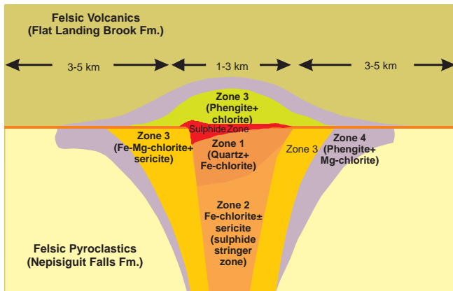
FIGURE 22. A schematic composite section through a VMS alteration system in the Bathurst mining camp as an example of a VMS proximal alteration zone metamorphosed to greenschist-grade mineral assemblages. From Goodfellow et al. (2003).
