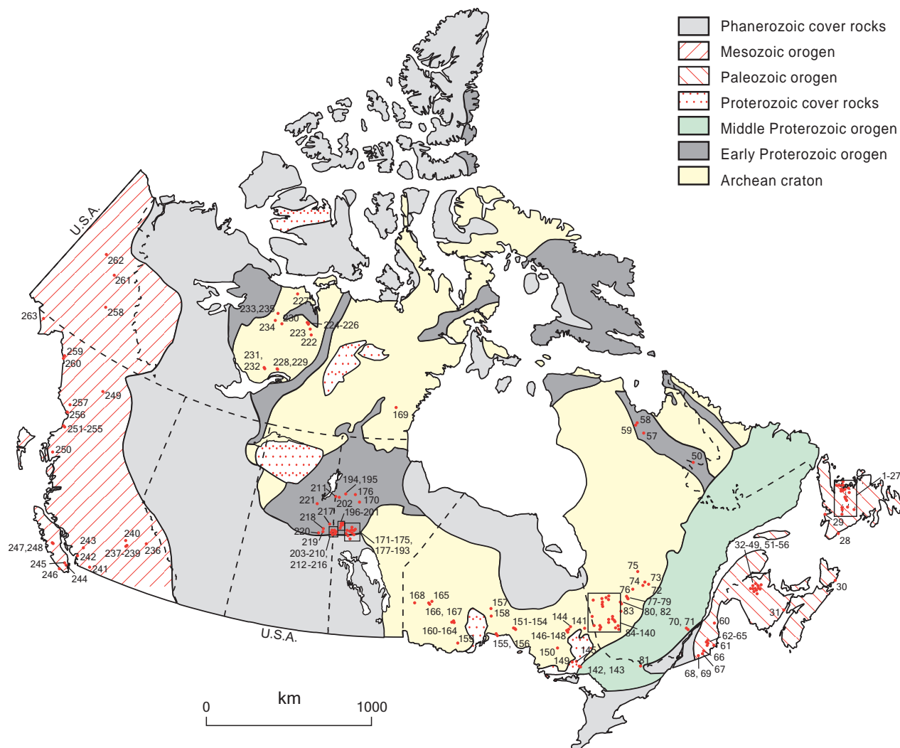
FIGURE 6. Distribution of VMS deposits in Canada by geologic province. Numbers correspond to deposits listed in the national VMS database (Appendix 1).
