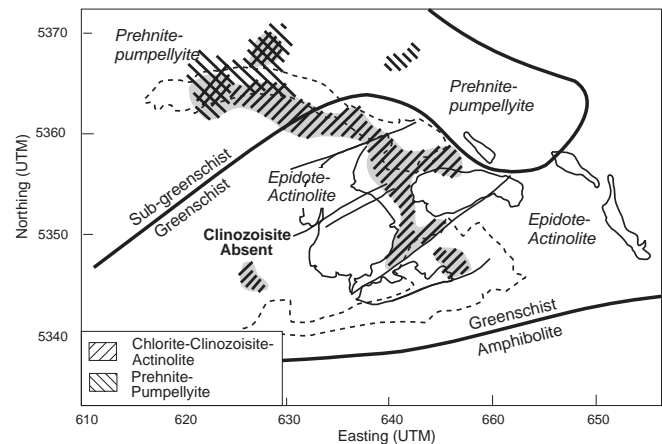
FIGURE 15. Comparison of regional greenschist-facies hydrothermal alteration in the Noranda Volcanic Complex with previously mapped metamorphic isograds (solid lines from Dimroth et al., 1983; Powell et al., 1993). The distribution of greenschist-facies hydrothermal alteration (shaded) suggests that interpreted metamorphic zonation is at least partly a product of early synvolcanic hydrothermal processes. Note that epidote and chlorite in the pre-cauldron sequence are distinct from those of the mine sequence volcanic rocks, even though they are well within the epidote-actinolite subfacies and have been metamorphosed at the same pressure and temperature. Modified from Hannington et al. (2003).
