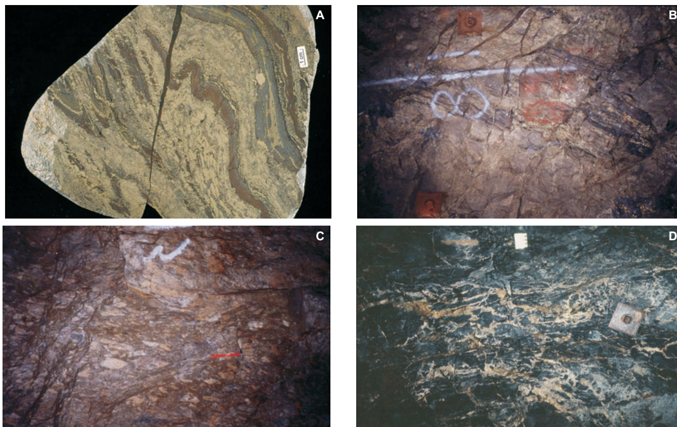
FIGURE 21. (A) Finely bedded tuff partially replaced by massive pyrrhotite-chalcopyrite at the Ansil deposit, Noranda. 15 cm metal plates for scale. (B) Cranston tuff unit with lit-par-lit replacement and in-filling by firstly by pyrite-sphalerite, followed by pyrrhotite-chalcopyrite, Ansil deposit, Noranda. (C) Rhyolite clasts cemented by pyrite-sphalerite rich sulphide groundmass, Louvicourt deposit, Val d'Or. 12 cm red magnet for scale. (D) Well developed pyrrhotite-chalcopyrite vein stockwork zone with intense chlorite alteration of the rhyolite wallrocks, Ansil deposit, Noranda.
