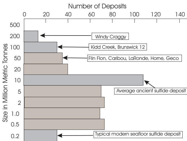
FIGURE 8. Global (proven, possible, and probable; non 43-101 compliant) size distribution for VMS deposits, with deposits over 50 Mt considered “very large” (Table 1), those over 100 Mt considered “giant”, and those over 150 Mt defined as “supergiant”. Atlantis II Deep, Red Sea, is considered the largest modern example of a seafloor massive sulphide deposit. Best known examples of Canadian very large, giant, and supergiant deposits are shown. Modified from Hannington et al. (1995).
