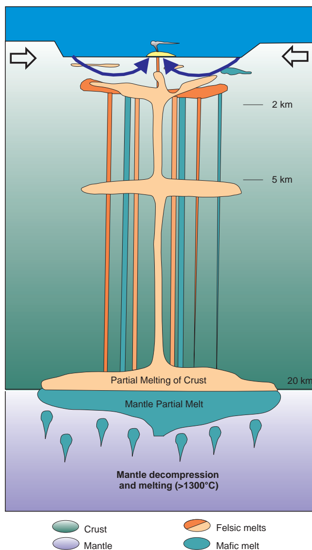
FIGURE 13. VMS environments are characterized by tectonic extension at various scales (open arrows). Extension resulted in crustal thinning, mantle depressurization, and the generation of basaltic melts. Depending on crustal thickness and density, these mafic melts ponded at the base of the crust, resulting in partial melting and generation of granitoid melts. These anhydrous, high-temperature melts quickly rose to a subseafloor environment (<3 km below seafloor), where their heat initiated and sustained convective hydrothermal cells that formed VMS deposits (black arrows).
