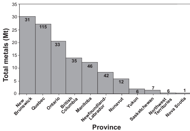
FIGURE 7. Histogram of the total tonnage of base metals from known VMS deposits per province; also shown are the number of deposits. The aggregate tonnage was calculated by total metals represent divided by geological reserves (proven, possible, and probable; non 43-101 compliant).
