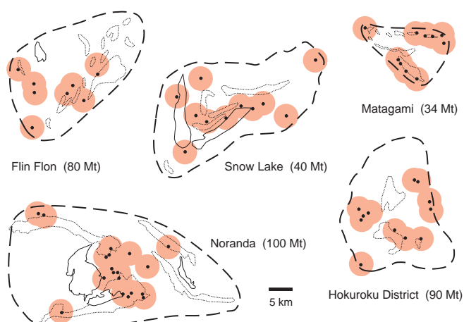
FIGURE 12. A same-scale comparison of selected VMS districts. A 5 km diameter circle around each deposit shows the hypothetical area of influence of proximal-scale alteration about each deposit, all encircled by a dashed line defining the proposed extent of a regional-scale alteration system for each camp based on the presence of known felsic volcanic and synvolcanic formations/intrusions (thin black lines). The Noranda example corresponds closely to the observed alteration. Modified from Sangster (1980).
