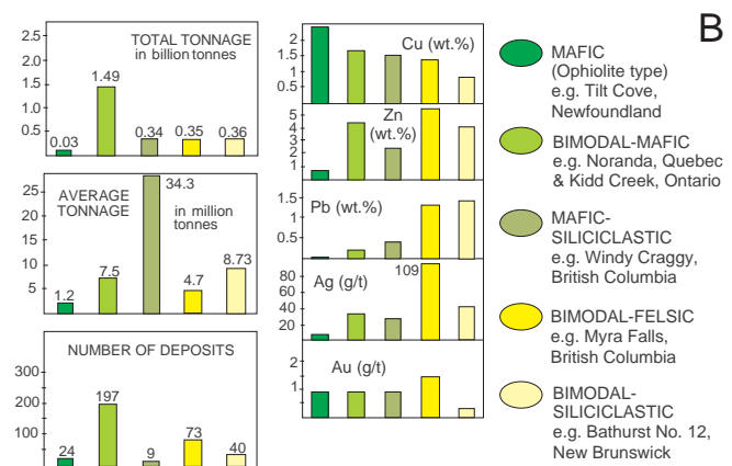
FIGURE 9. Statistics for VMS deposits grouped by lithologic class (Barrie and Hannington, 1999): (A) worldwide deposits; (B) Canadian deposits.
