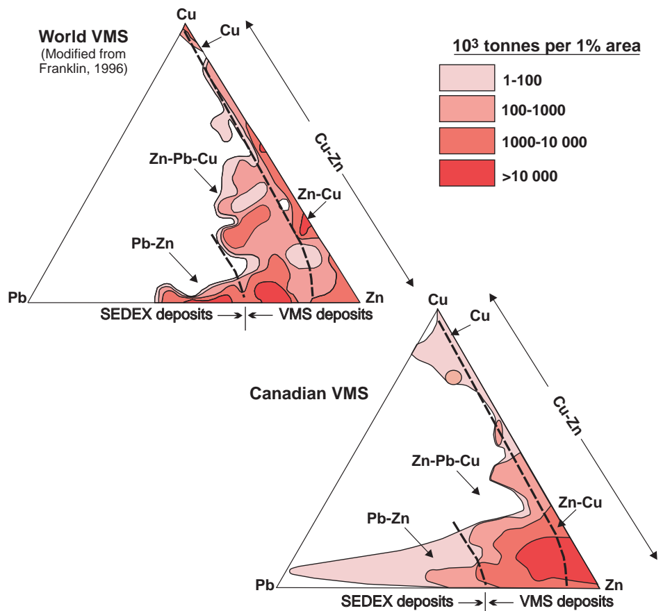
FIGURE 2. Base metal classification scheme of worldwide and Canadian VMS deposits as defined by Franklin et al. (1981) and modified by Large (1992) to include the Zn-Pb-Cu class. The preponderance of Cu-Zn and Zn-Cu VMS deposits in Canada is due to the abundance of Precambrian primitive oceanic arc settings. Worldwide, there is a larger proportion of felsic-hosted, more Pb-rich continental rift and continent margin arc settings.
