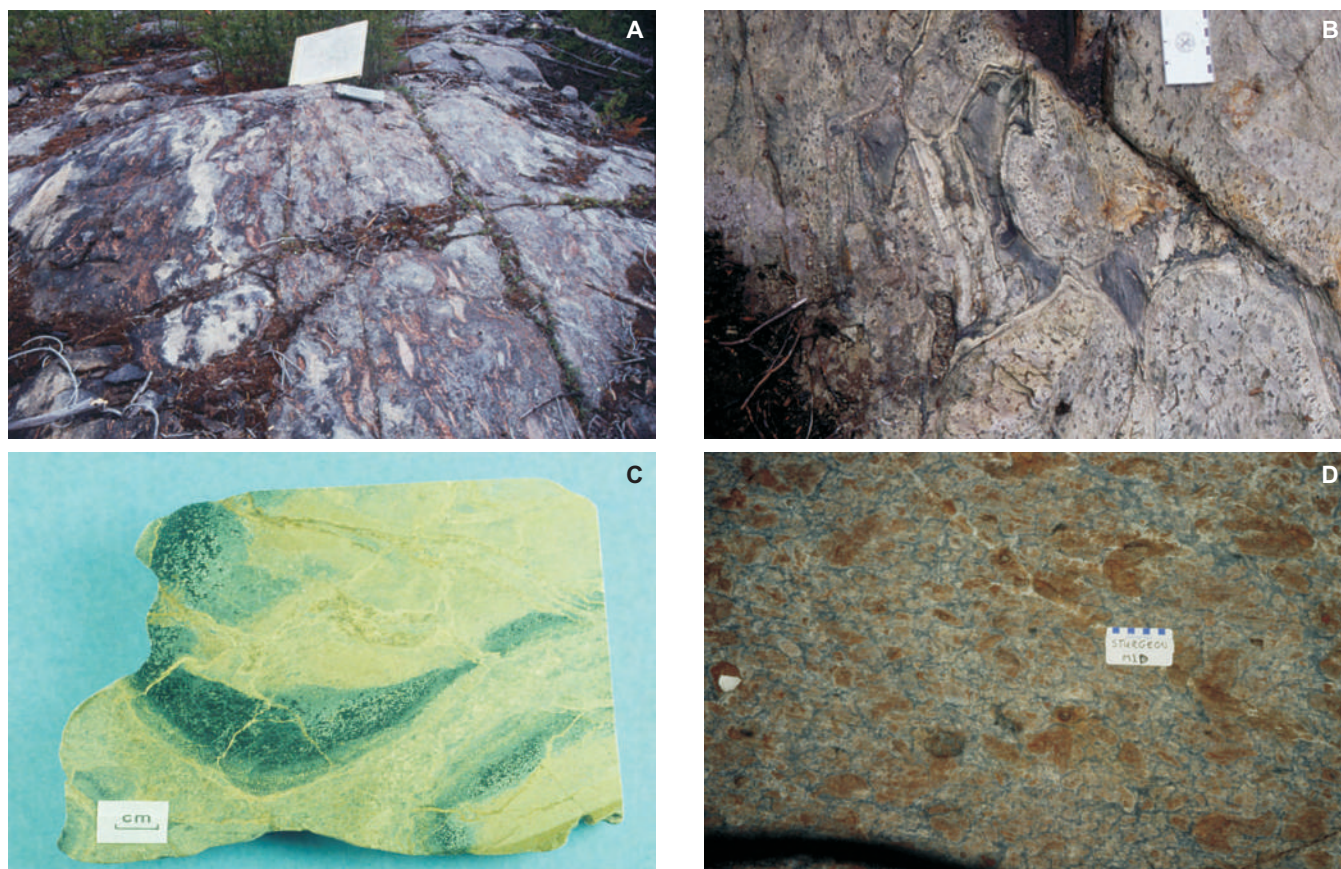
FIGURE 16. (A) High-temperature hydrothermally altered mafic volcanoclastic turbidite (left) overlain by a strongly silicified mafic debris flow 1200 m below the Chisel-Lost-Ghost VMS horizon, Snow Lake. This is a regional-scale reaction zone overlain by a high-temperature zone of silica precipitation. (B) Strongly silicified pillows with pipe vesicles infilled with actinolite, epidote, and magnetite, and interpillow hyaloclastite completely replaced by the same assemblage. This alteration facies directly overlies the subvolcanic Mooshla intrusion, Bousquet VMS camp, Quebec. (C) Epidosite typical of the root zones of VMS hydrothermal upflow zones in which high fluid/rock ratios have resulted in leaching of lithophile, chalcophile, and low field strength elements from the strata. (D) Chloritoid-rich zone below the Matabi deposit, Sturgeon Lake, where Fe-rich hydrothermal fluids overprinted a previously formed carbonate-rich regional alteration zone.
