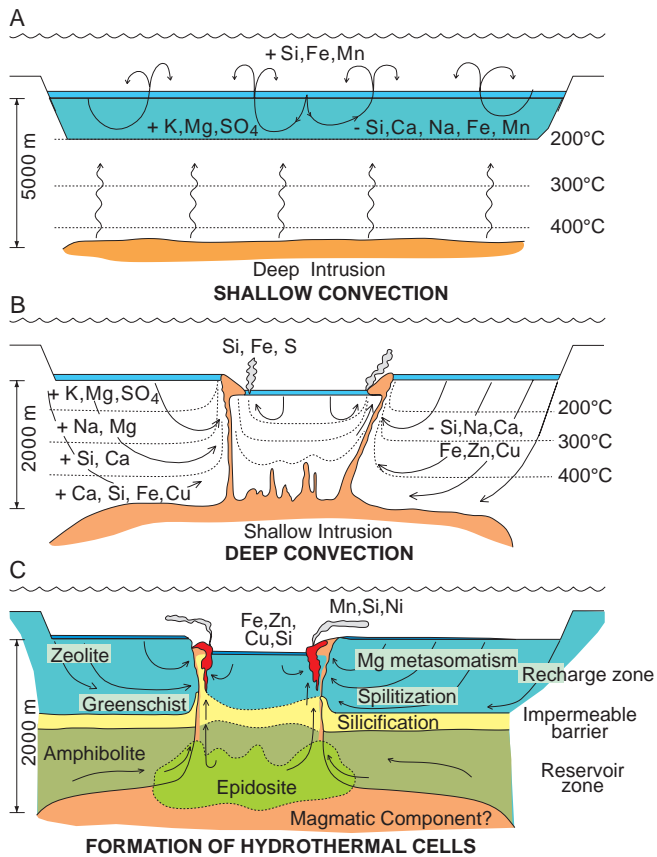
FIGURE 14. The development and maturation of a generic subsurface hydrothermal system involves three stages. (A) The relatively deep emplacement of a subvolcanic intrusion below a rift/caldera and the establishment of a shallow circulating, low-temperature seawater convection system. This results in shallow subsurface alteration and associated formation of hydrothermal exhalative sediments. (B) Higher level intrusion of subvolcanic magmas and resultant generation of a deep-seated subsurface seawater convection system in which net gains and losses of elements are dictated by subhorizontal isotherms. (C) Development of a mature, large-scale hydrothermal system in which subhorizontal isotherms control the formation of semiconformable hydrothermal alteration assemblages. The high-temperature reaction zone next to the cooling intrusion is periodically breached due to seismic activity or dyke emplacement, allowing focused upflow of metal-rich fluids to the seafloor and formation of VMS deposits. From Galley (1993).
