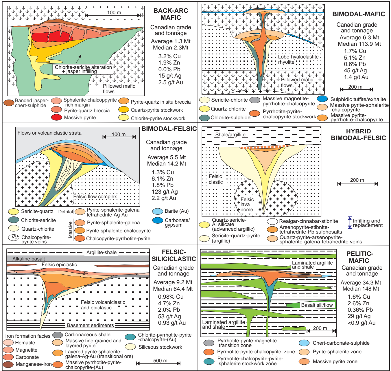
FIGURE 4. Graphic representation of the lithological classifications modified from Barrie and Hannington (1999) by Franklin et al. (2005), with the addition of the hybrid bimodal felsic as a VMS-epithermal subtype of bimodal-felsic. Average and median sizes for each type for representative Canadian deposits shown, along with average grade.
