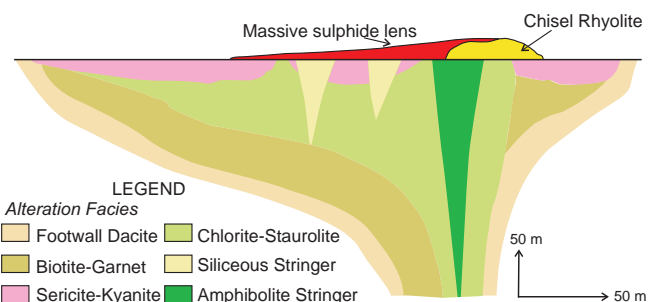
FIGURE 23. A stylized cross-section through the proximal alteration zone at the Chisel deposit, Snow Lake mining camp, illustrating the changes in mineral assemblages that occur when the terrane undergoes lower to middle amphibolite-grade regional metamorphism. From Galley et al. (1993).
