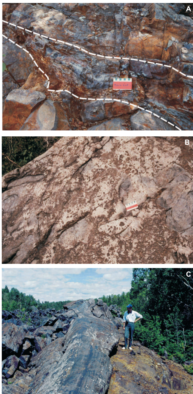
FIGURE 18. (A) Mine contact tuff exhalite horizon (between white lines) that overlies the silicified andesites of the Waite Formation, Noranda, Quebec. (B) Silicified basaltic andesite of the Upper Amulet Formation., Noranda, Quebec, as an example of pervasive silica precipitation that occurred in mafic flows directly underlying tuffaceous exhalite units in many Precambrian VMS camps. (C) Banded magnetite-chert Fe-formation overlying the Austin Brook massive sulphide deposit, Bathurst camp (photo by J.M. Peter).
