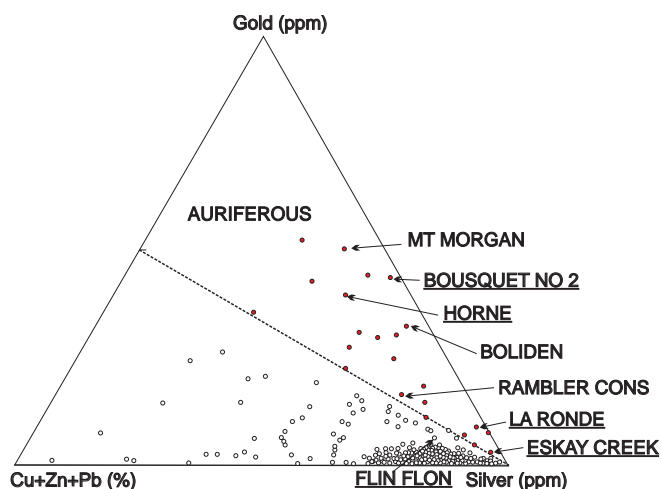
FIGURE 3. Classification of VMS deposits based on their relative base metal (Cu+Zn+Pb) versus precious metal (Au, Ag) contents. Some of Canada’s better known auriferous deposits (underlined) are compared to international examples. Despite having produced 170 t of Au, the Flin Flon deposit is not considered an auriferous VMS deposit under this classification. Modified from Hannington et al. (1999c).
